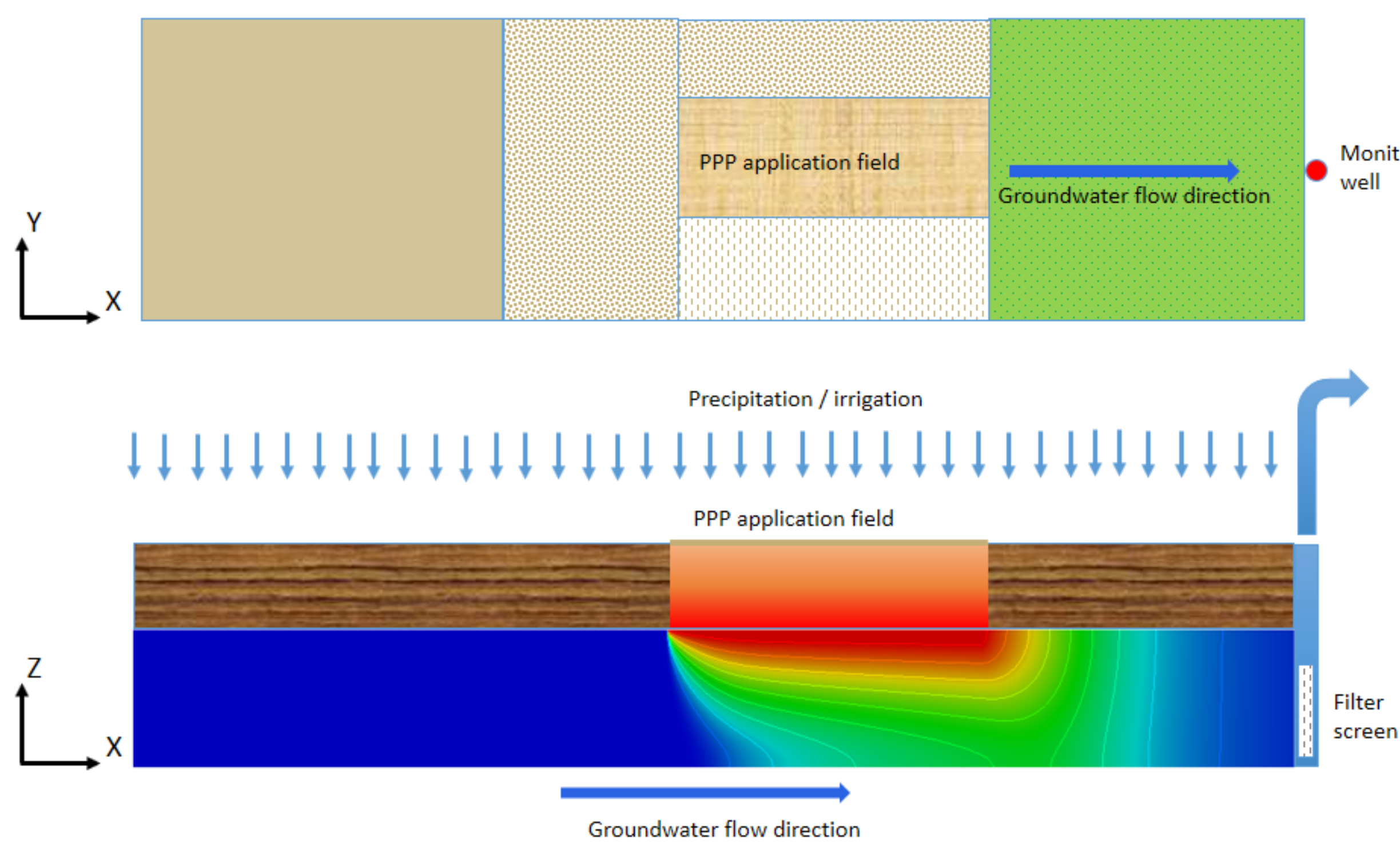
Figure 1 Schematic representation of PPP transport in the subsurface below a treated field
